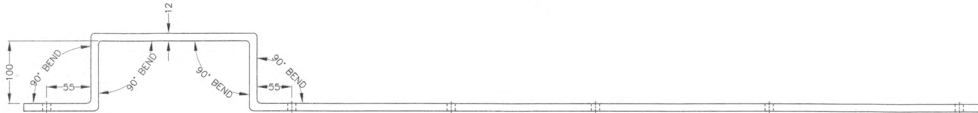
ELEVATION (RDSO/T- 9010)
